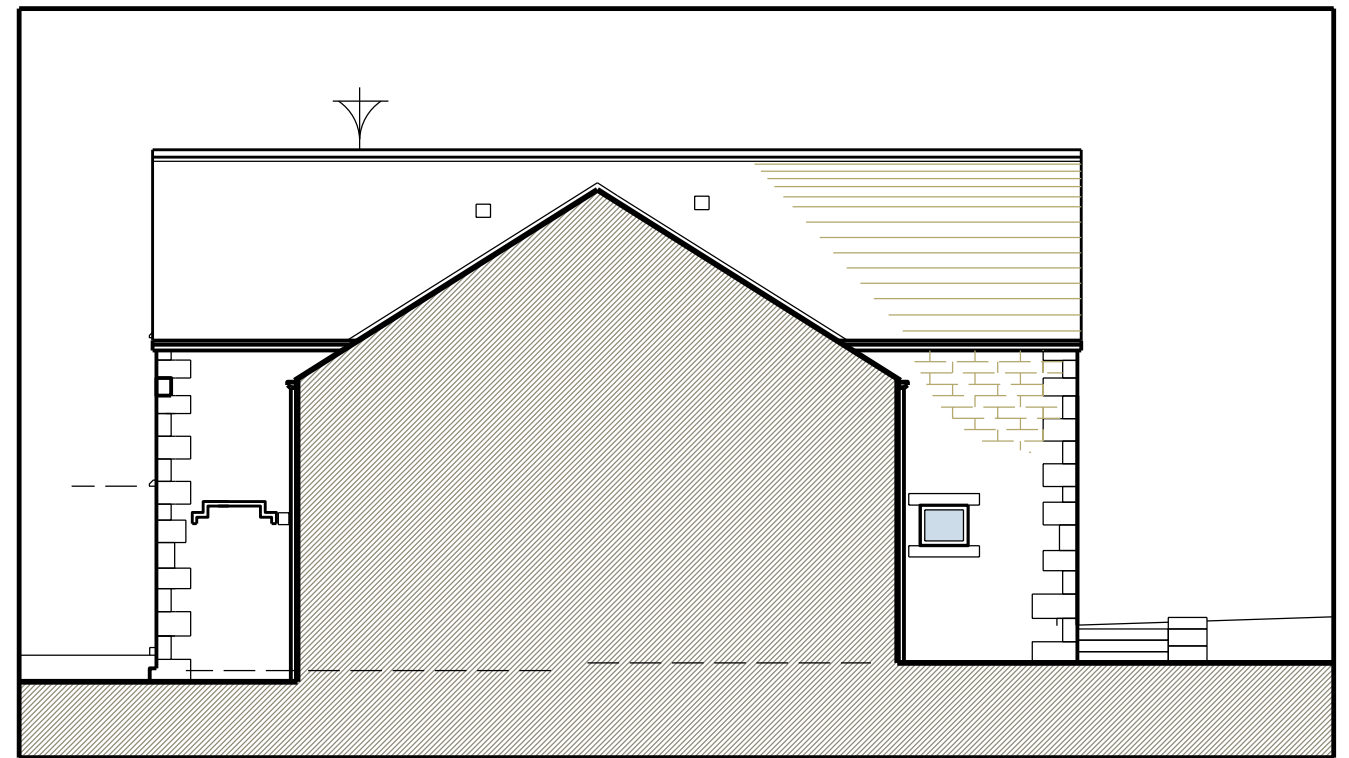
East Elevation
