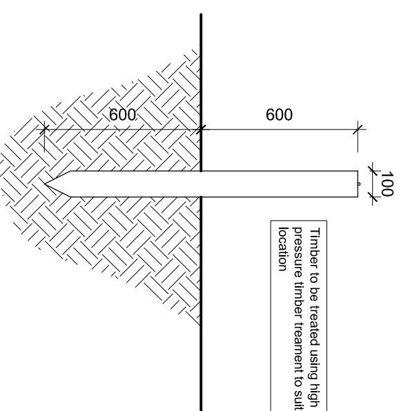
TYPICAL SECTION 1:20
