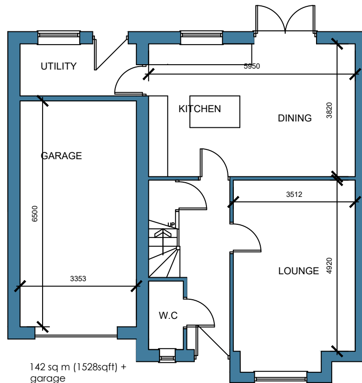
GROUND FLOOR PLAN PLOTS 8,9 & 10 SHOWN. PLOT 7 HANDED
