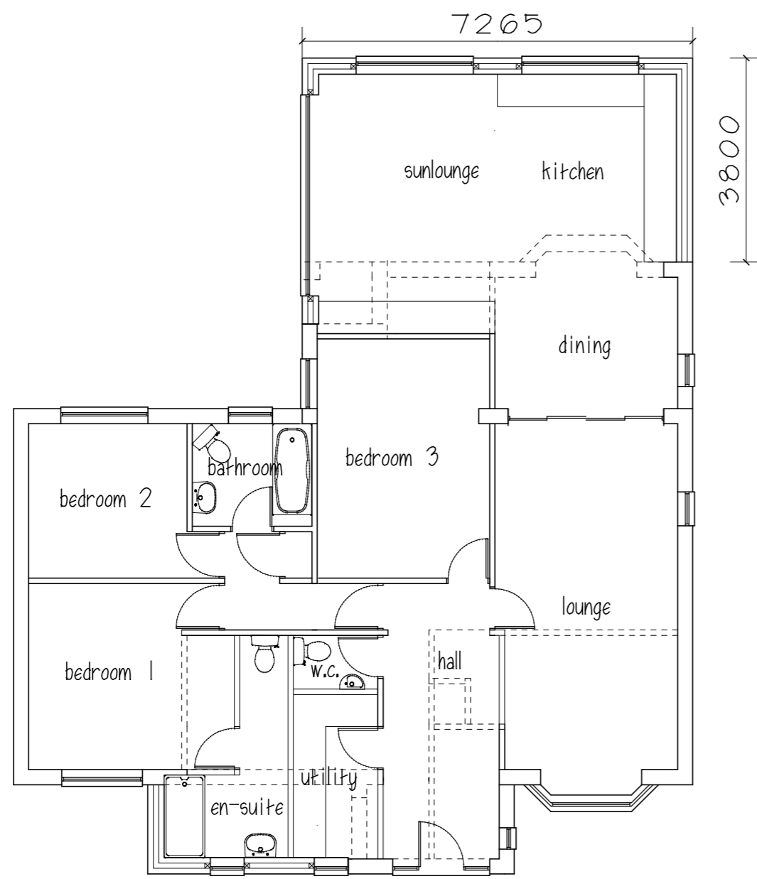
GROUND FLOOR
