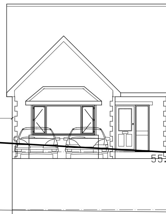
FRONT ELEVATION
