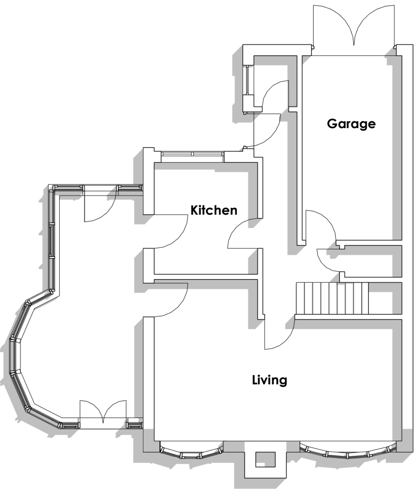
Ground Floor 1 : 100
