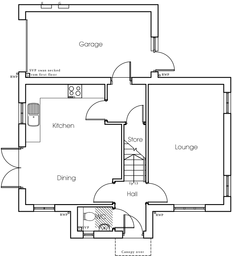
Ground Floor Scale - 1:100
