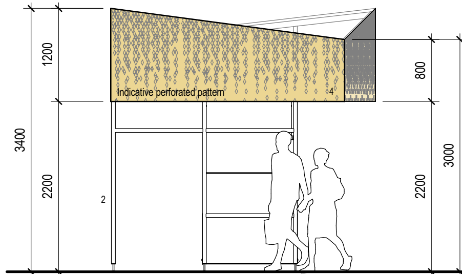
Proposed Elevation D (Folded Countertop) 1:50
