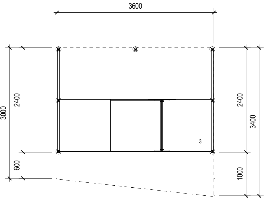
Proposed Plan 1:50
