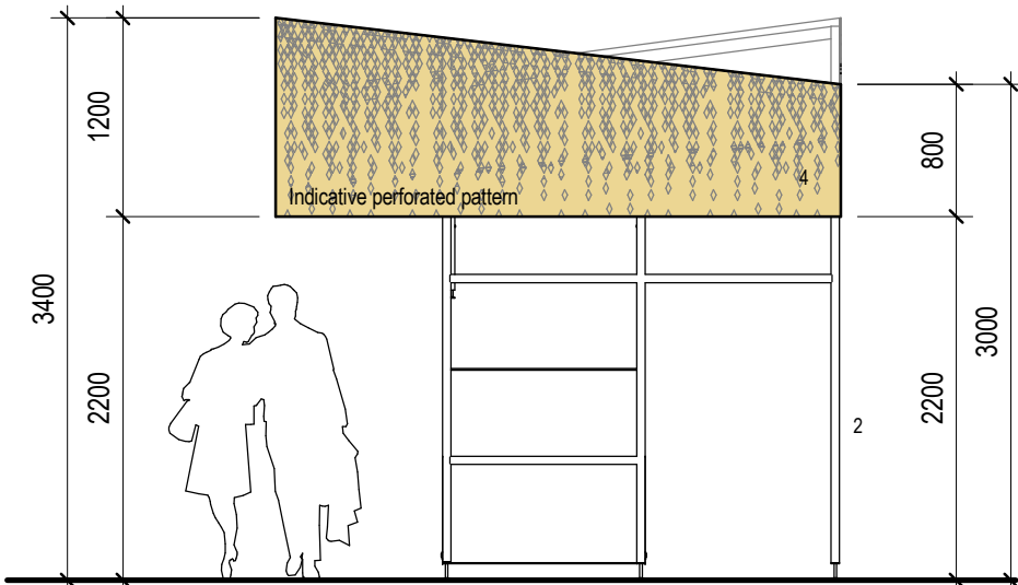
Proposed Elevation C (Folded Countertop) 1:50
