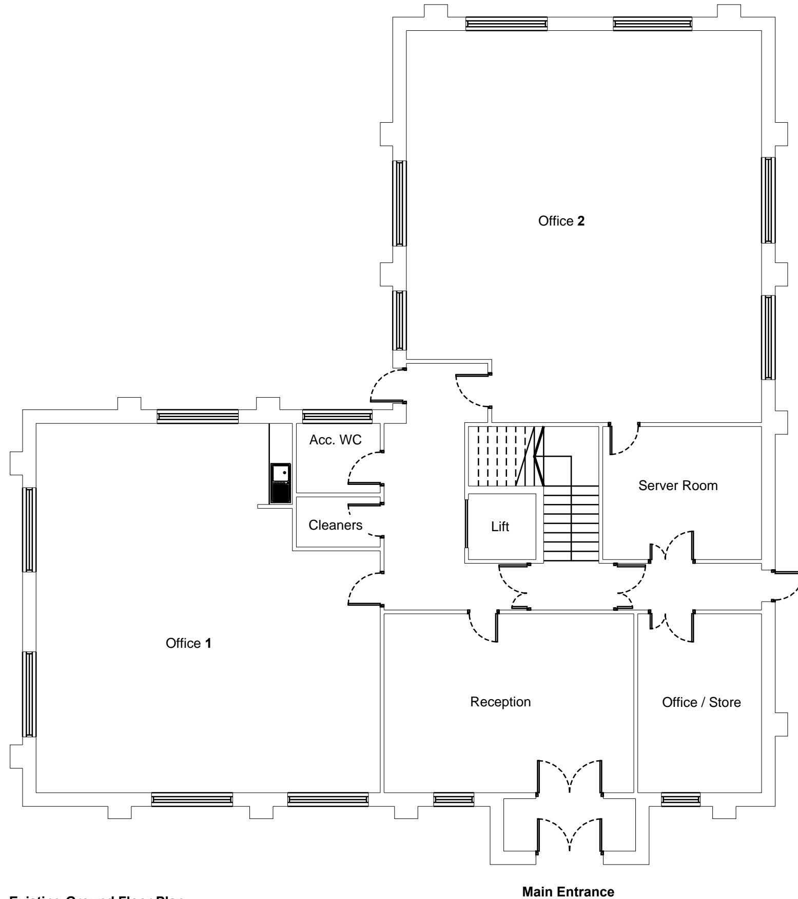
Existing Ground Floor Plan Phoenix House Tankersley
