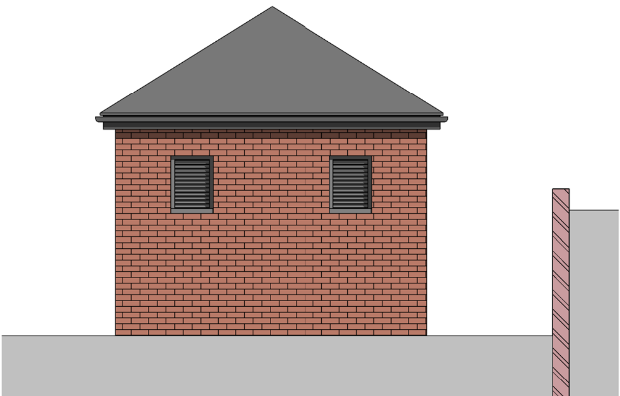
Elevation C (West) 1 : 50
