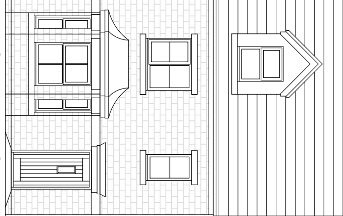
FRONT ELEVATION PLOTS 25 to 27
