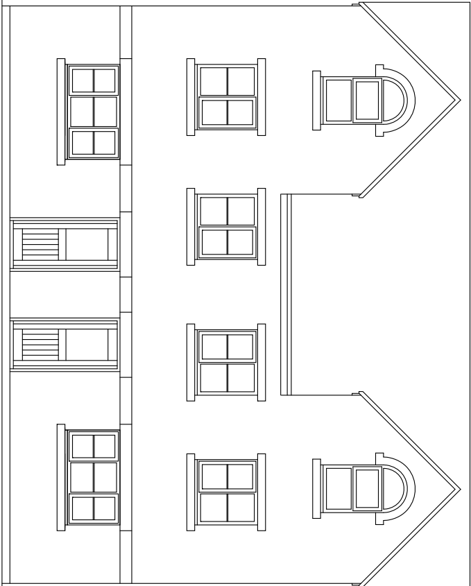
REAR ELEVATION - Plots 18-19
