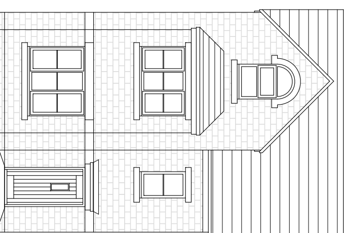
FRONT ELEVATION - PLOT 28
