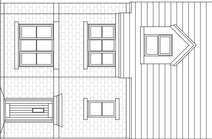
FRONT ELEVATION - PLOT 28
