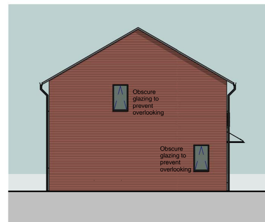
Plot 30 Side / West Elevation 1 : 100
