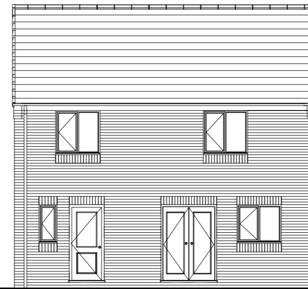
REAR ELEVATION
