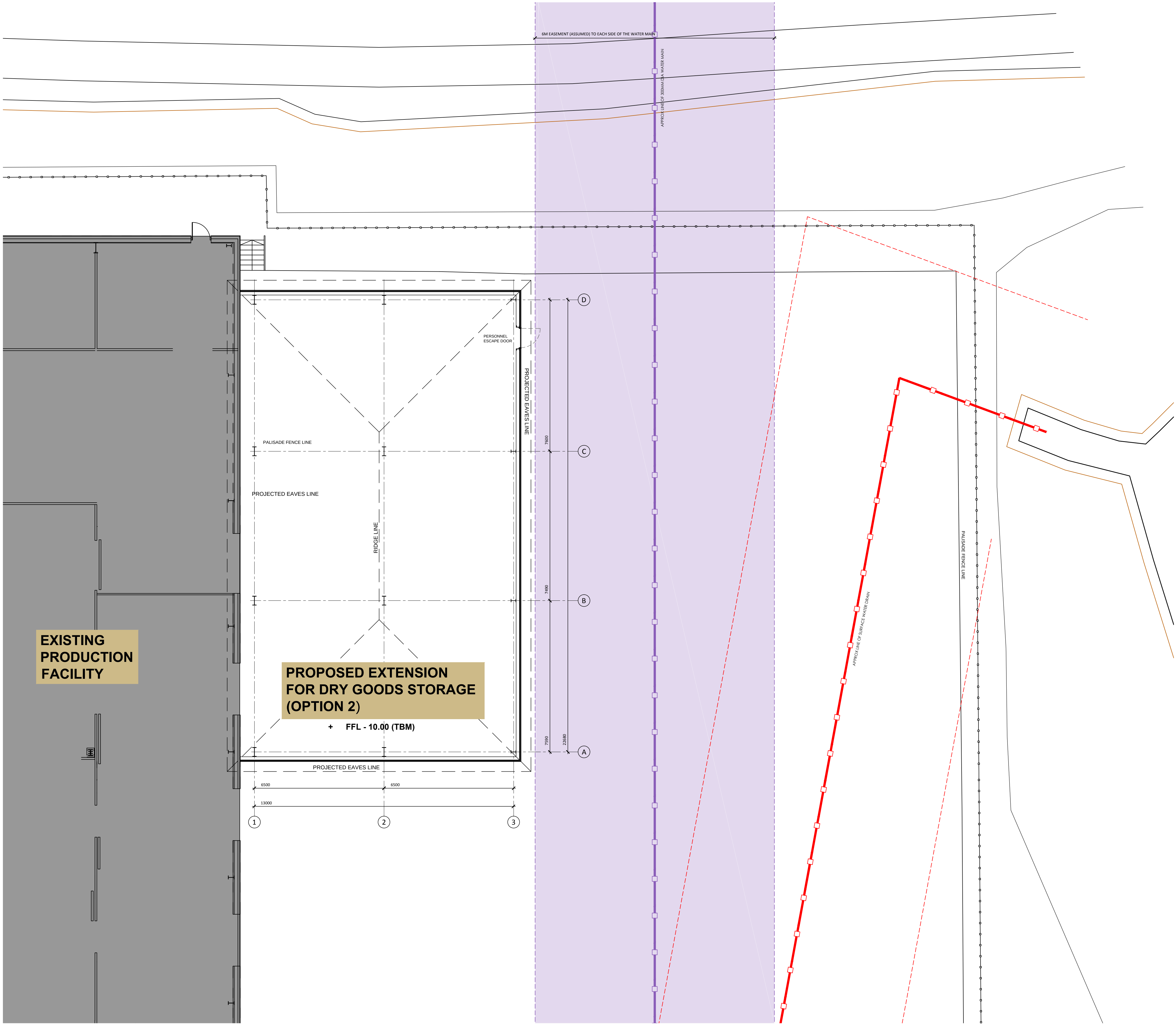
PROPOSED BUILDING PLAN SCALE: 1:100
