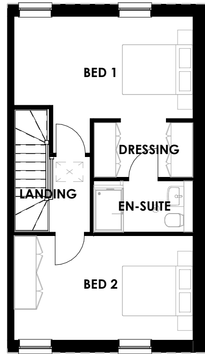
SECOND FLOOR PLANNING 1 : 100
