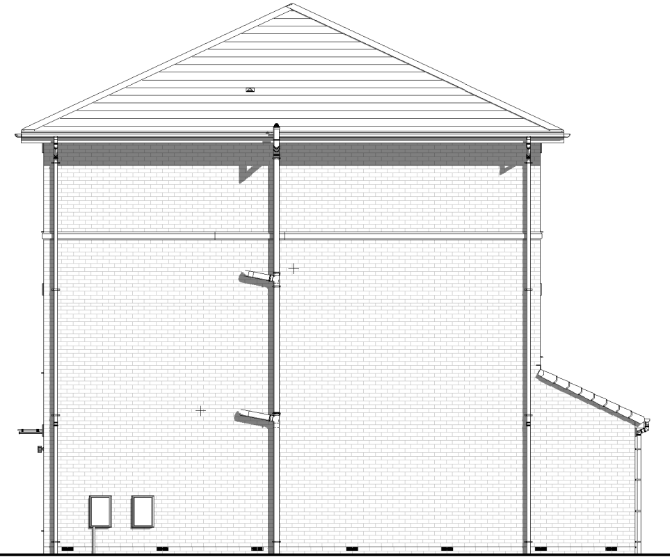
ELEVATION B PLANNING 1 : 100
