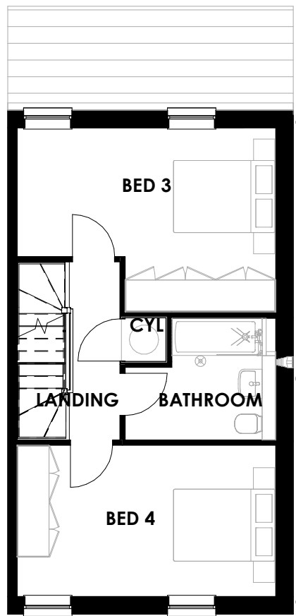
FIRST FLOOR PLANNING 1 : 100
