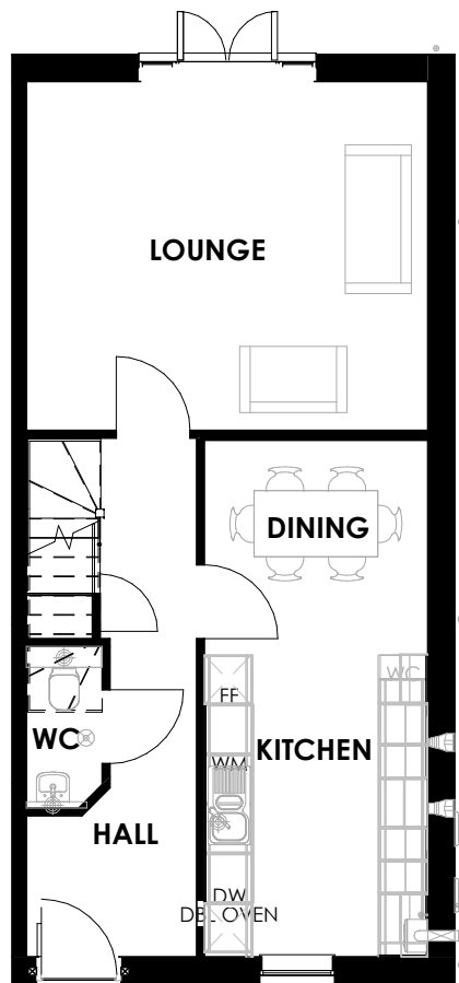
GROUND FLOOR PLANNING 1 : 100
