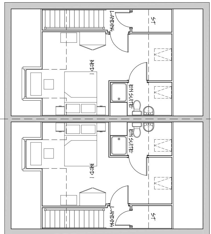
Second Floor Layout
