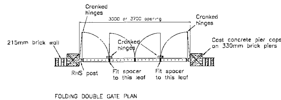
FOLDING DOUBLE GATE PLAN
