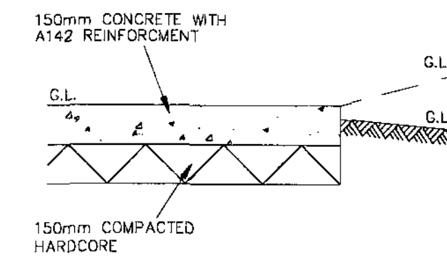
CONCRETE DRIVE WITH LITTLE OR NO DIFFERENCE IN LEVEL SCALE 1:20
