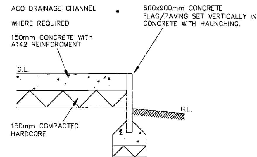
CONCRETE DRIVE WITH DIFFERENCE IN LEVEL BETWEEN LEVEL-600MM SCALE 1:20
