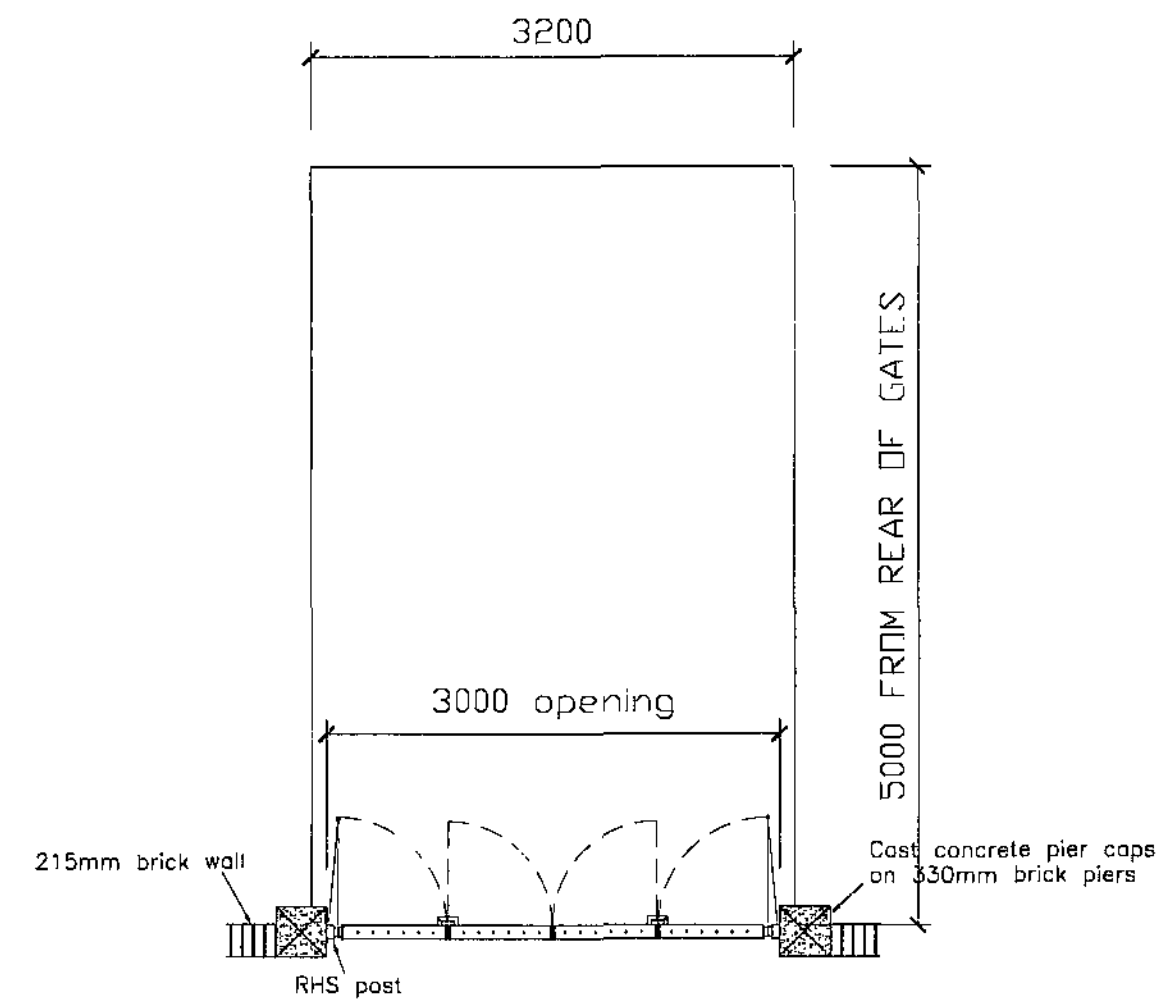
DRIVE DOUBLE GATE PLAN SETTING OUT SCALE 1:50
