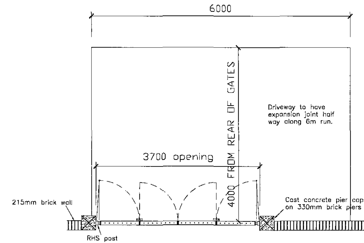
DRIVE DOUBLE GATE PLAN ALTERNATIVE SETTING OUT SCALE 1:50
