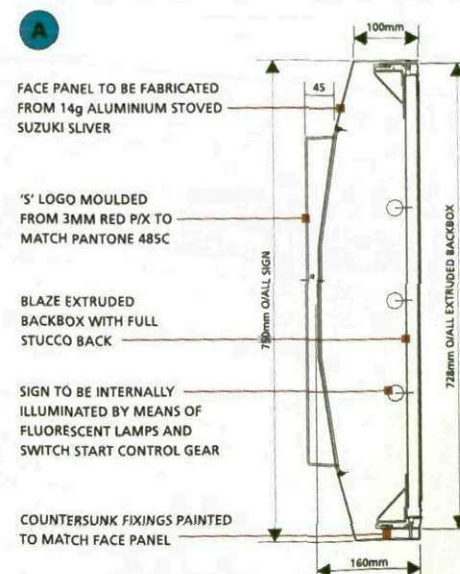
SECTION DETAIL
