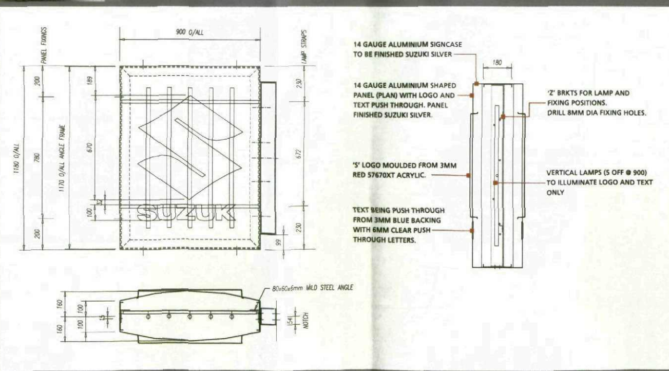
SECTION DETAIL
