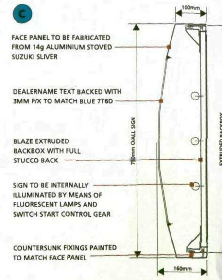
750mm DEEP ROLLED FASCIA - SCALE 1:10 @ A3
