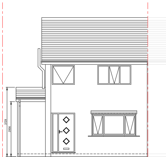
FRONT ELEVATION
