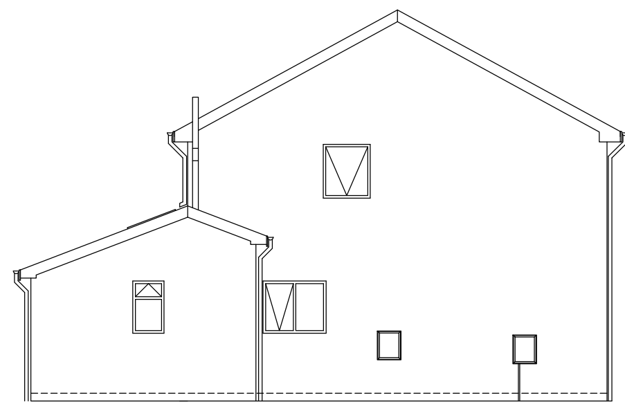
LEFT HAND ELEVATION (FROM 5 PINFIELD CLOSE)
