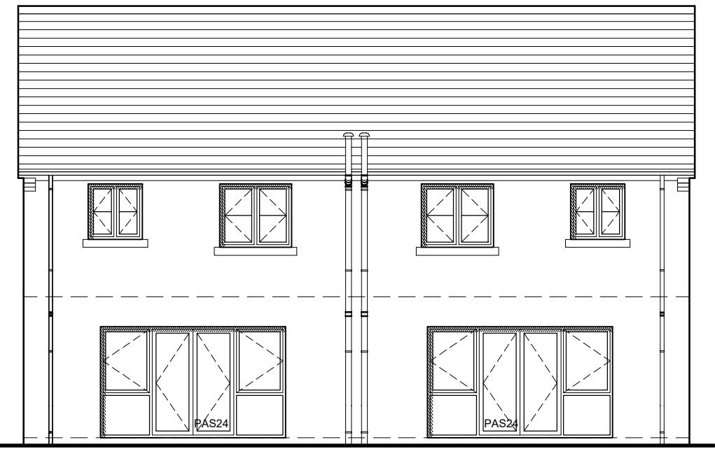
REAR ELEVATION
