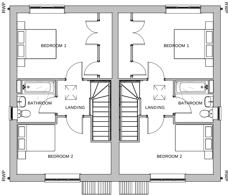
First Floor 1 : 100
