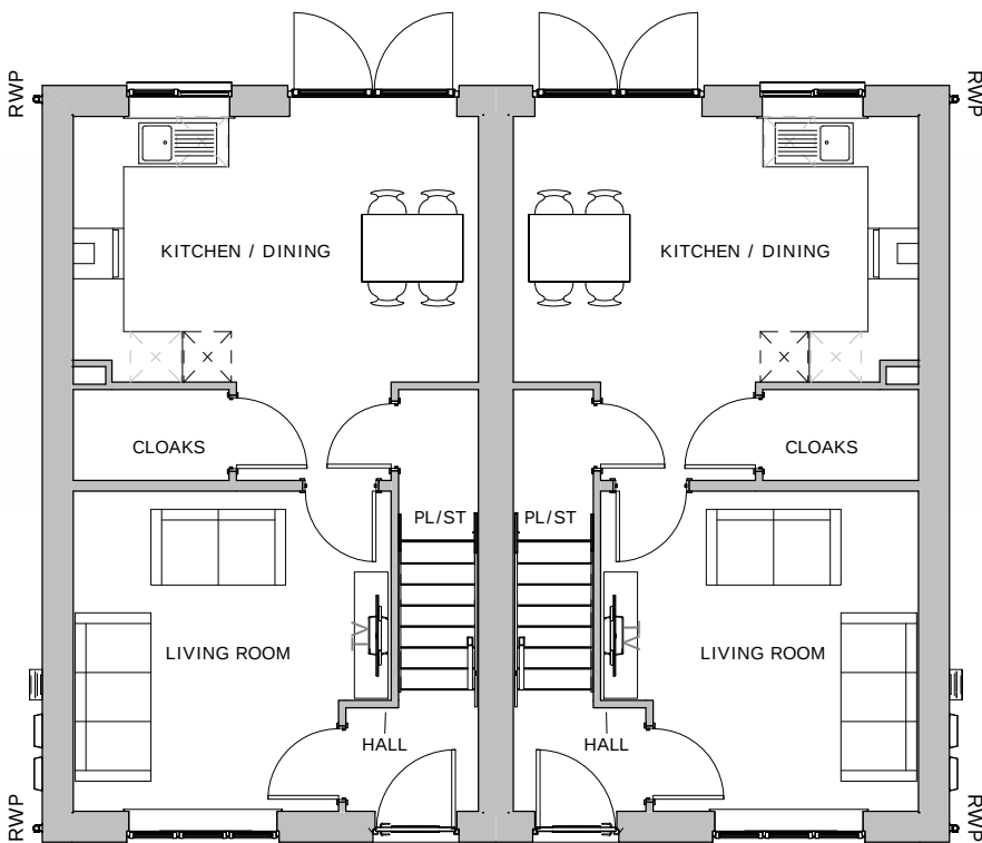
Ground Floor 1 : 100
