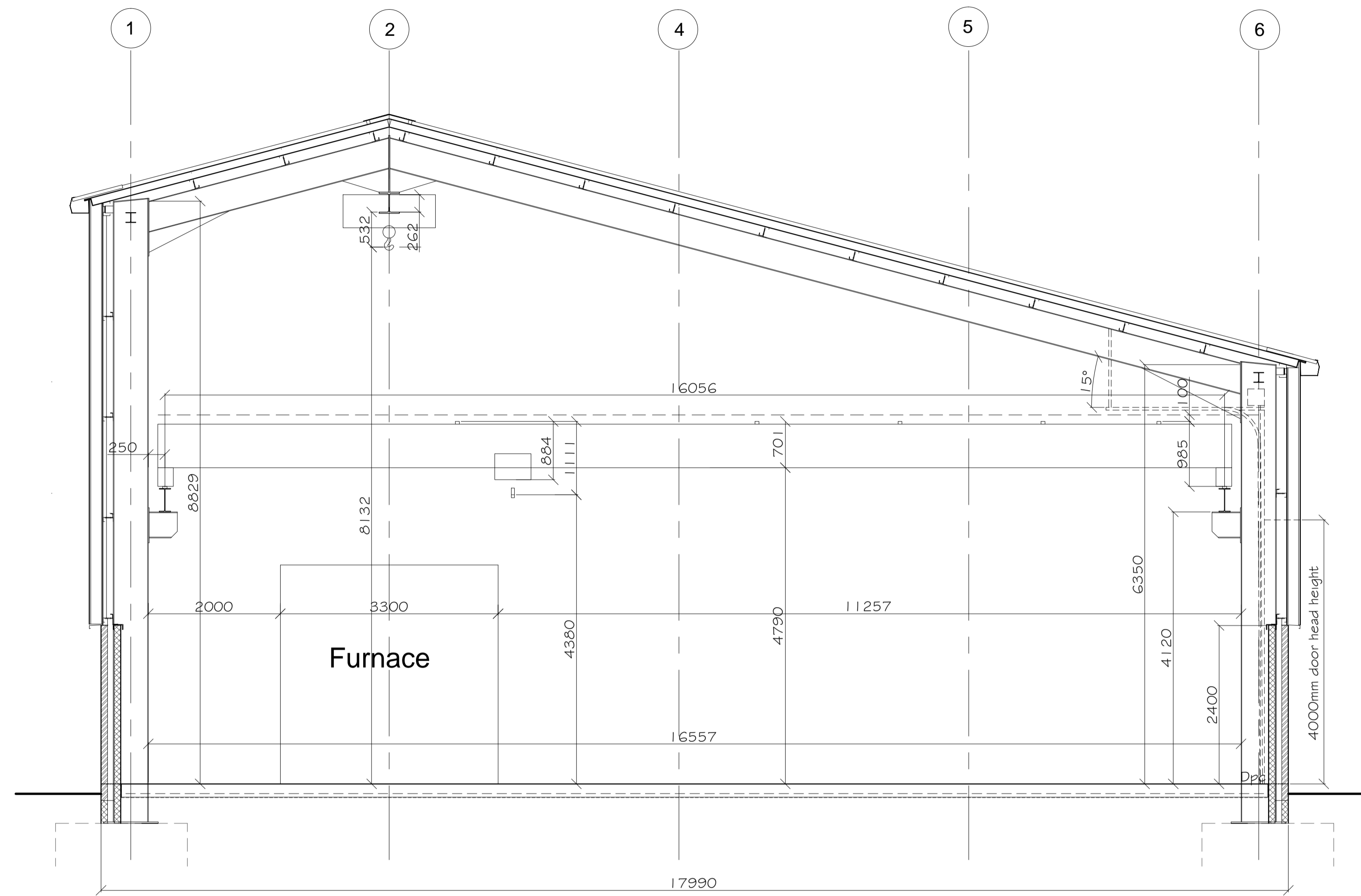
SECTION SCALE 1:100
