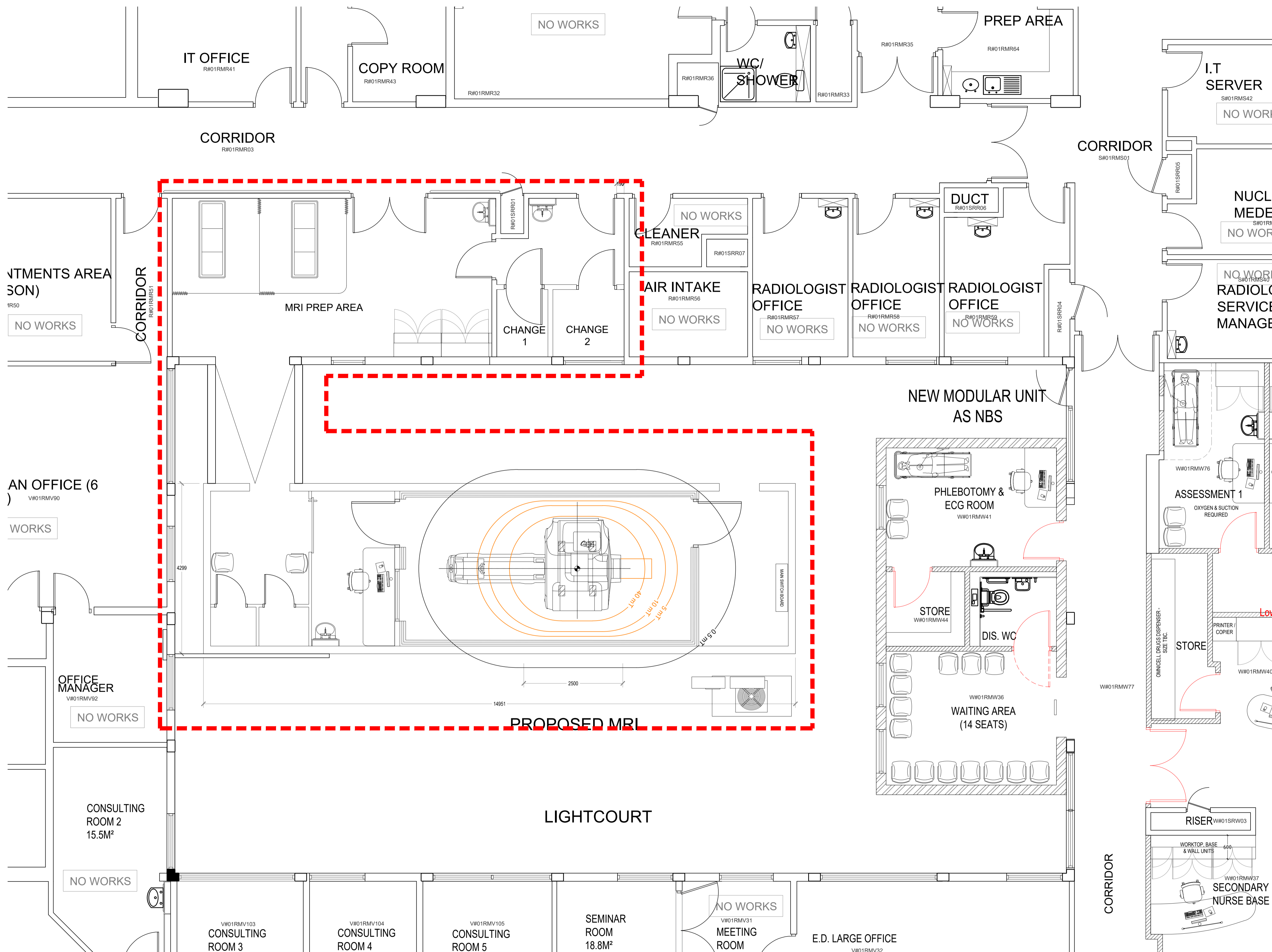
PROPOSED PLAN 1:50
