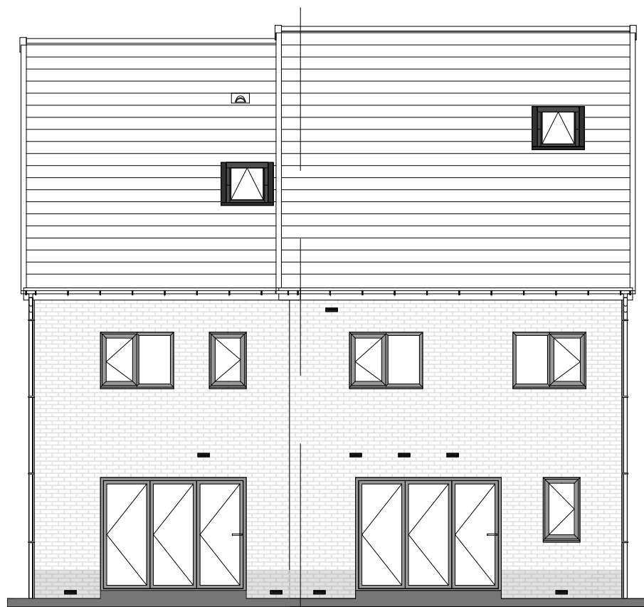
REAR ELEVATION
