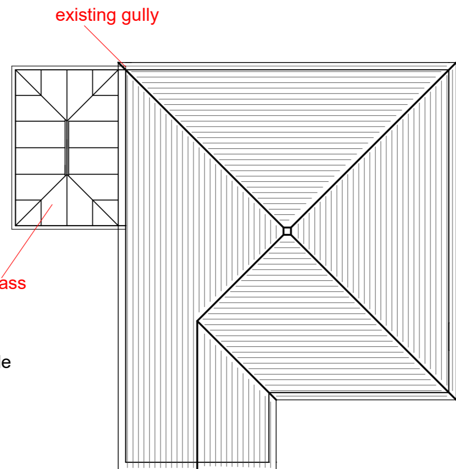
ROOF PLAN
