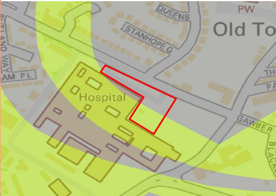
Figure 6: Solid geology
