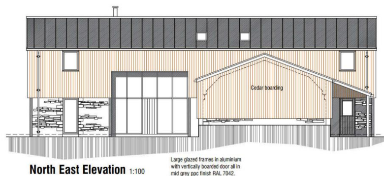
Fig 12. Typical elevation of converted barn.
