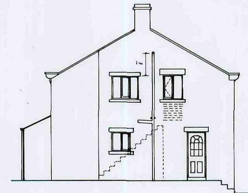
WEST ELEVATION
