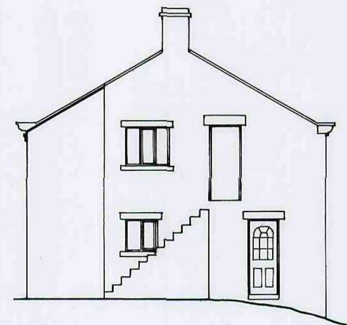
WEST ELEVATION
