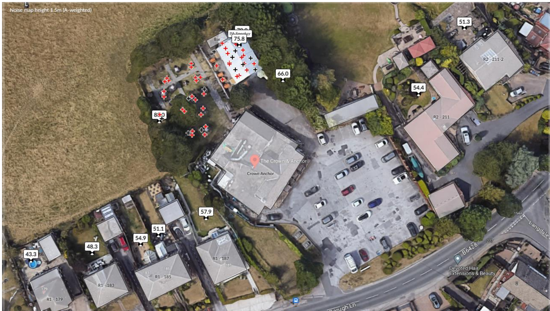
Figure 4: Predicted maximum sound levels of 10 people using raised voices - L_{AFmax}
