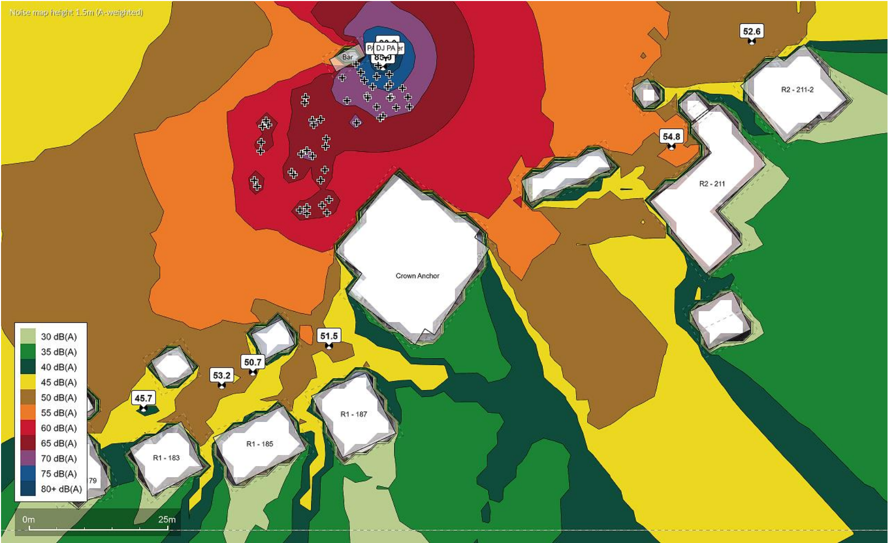
Figure 3: Scenario C equivalent sound level map - L_{Aeq,1hour}
