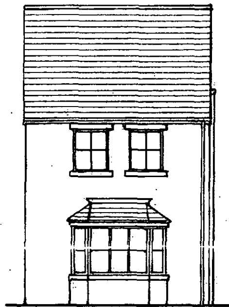
FRONT ELEVATION
