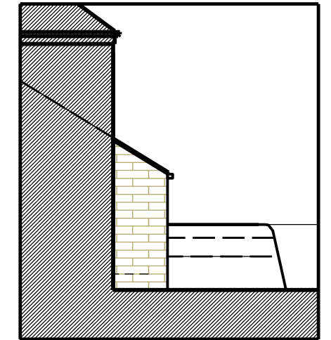
West Elevation - Proposed
