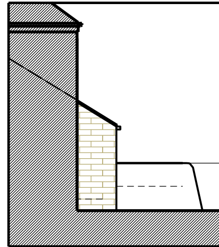
West Elevation - Existing
