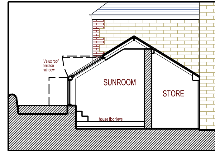
East Elevation/ Section - Proposed
