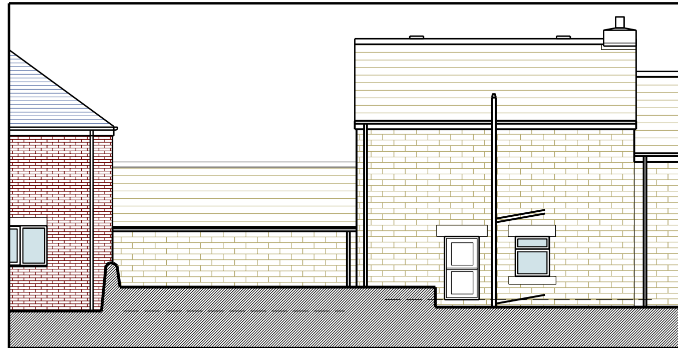
South Elevation - Existing
