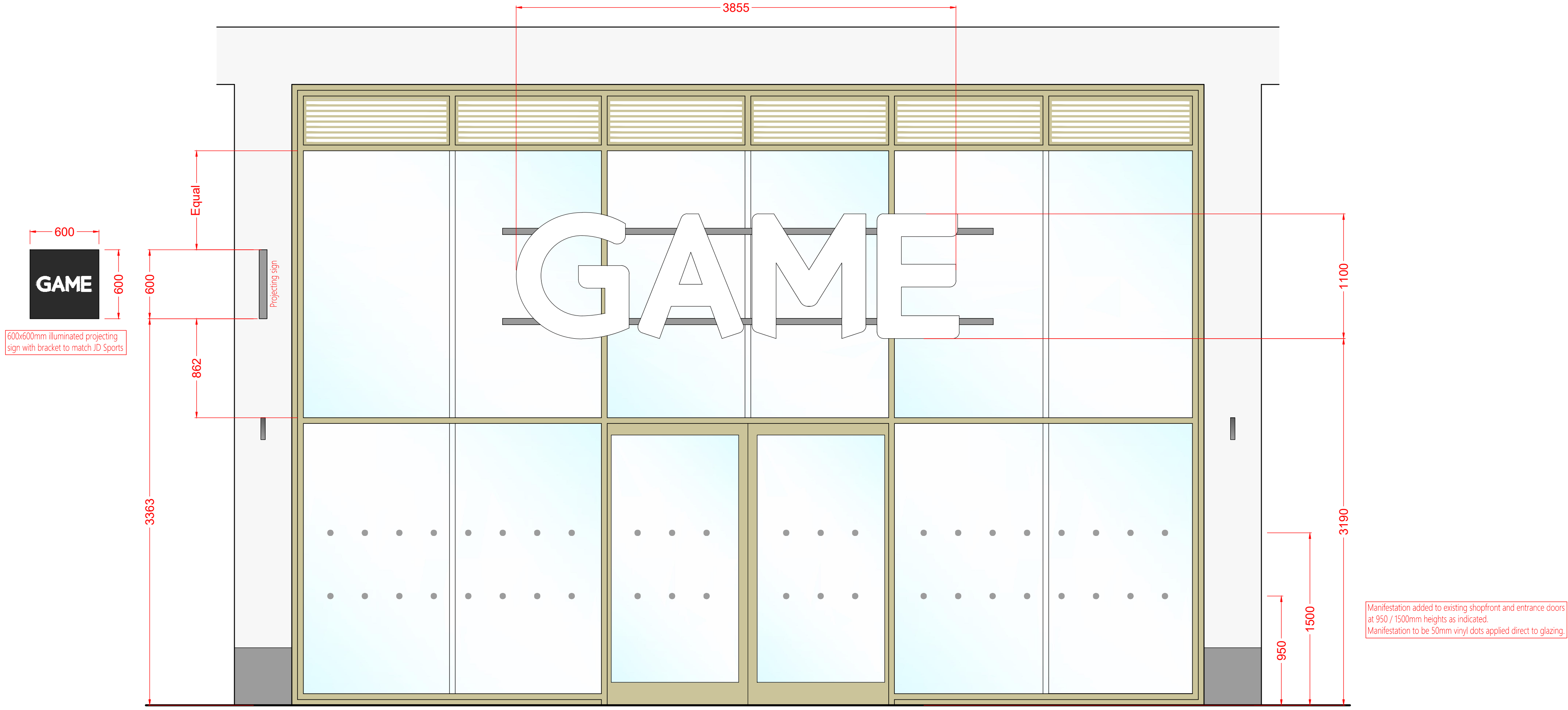
PROPOSED SHOPFRONT (1:25)
