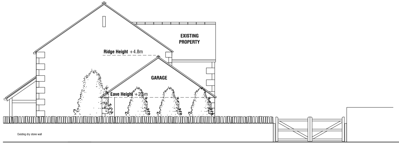
REAR ELEVATION 1:100
