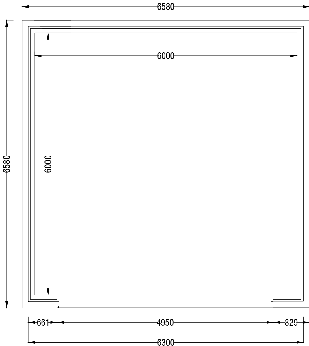
FLOOR PLAN 1:50
