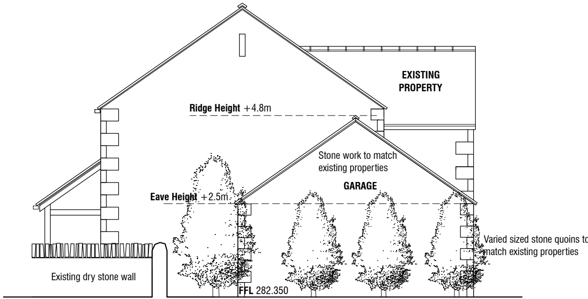
SIDE ELEVATION 1:100
