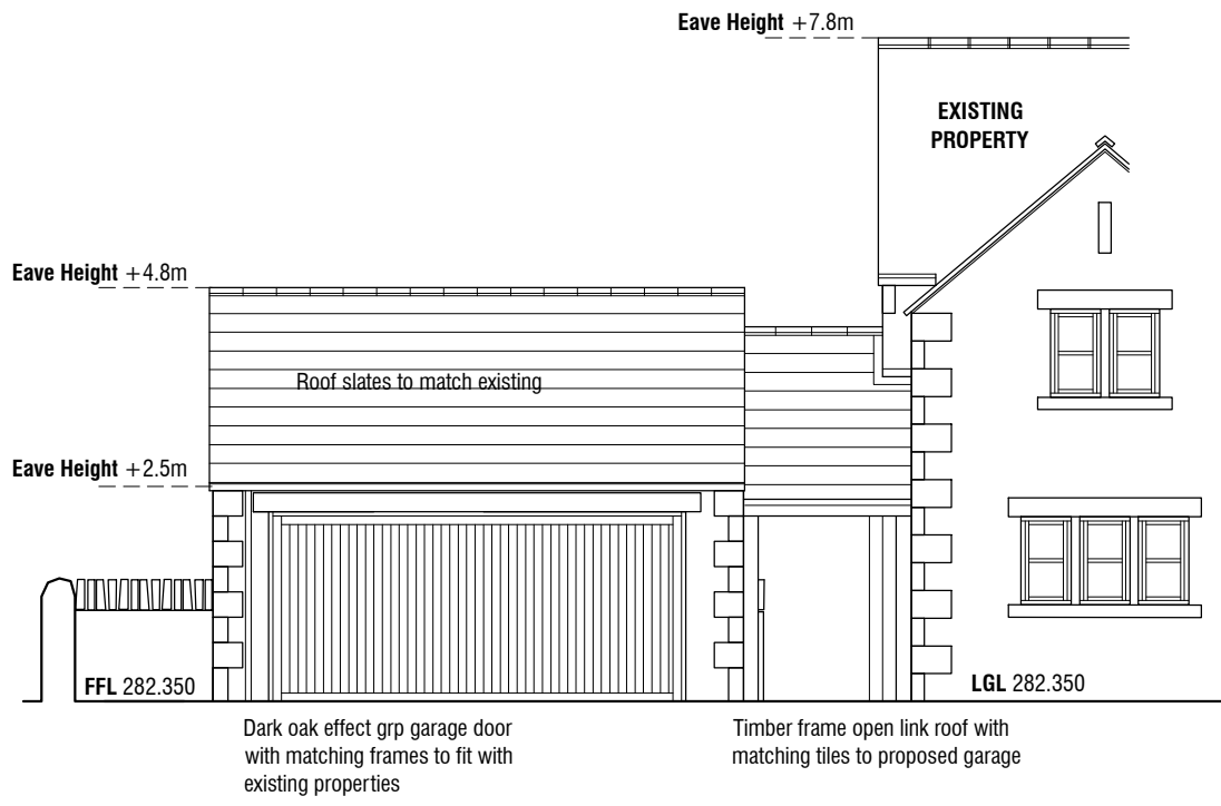
REAR ELEVATION 1:100
