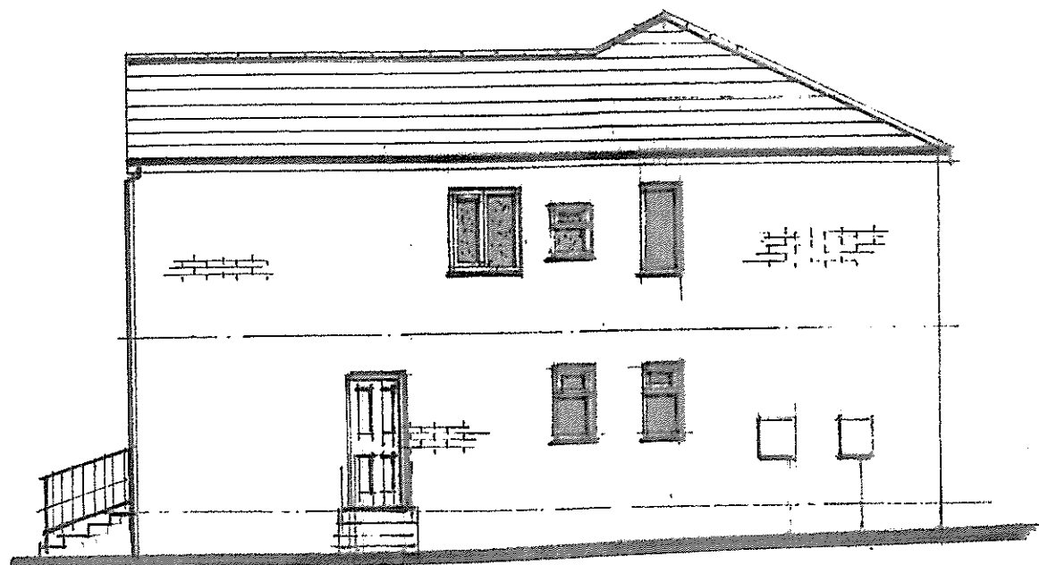
Proposed Side Elevation On 2
