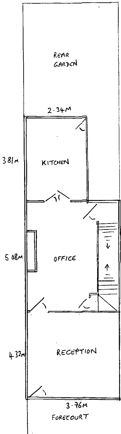
GROUND FLOOR
