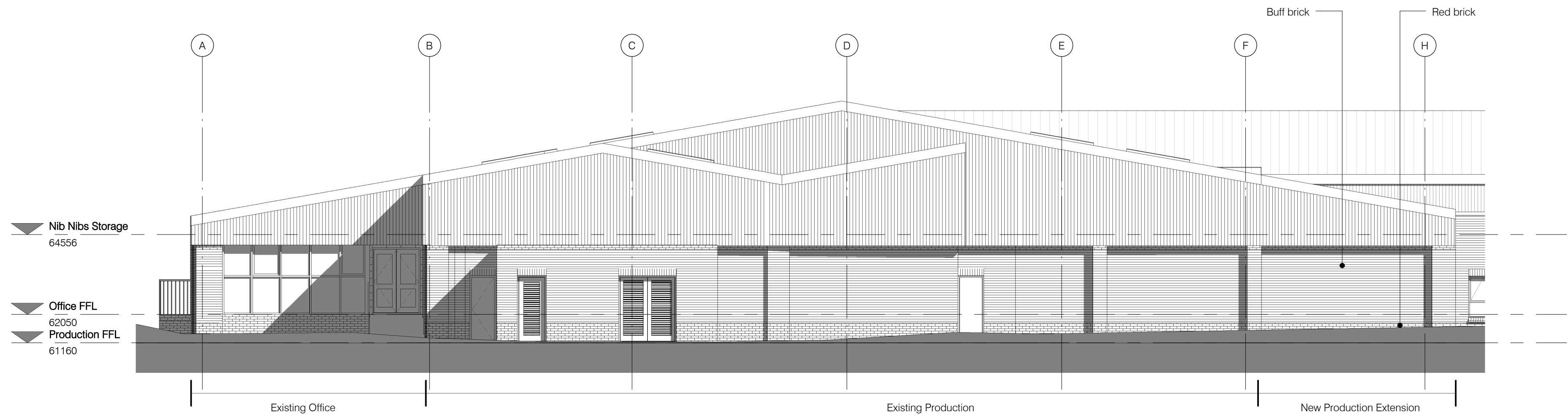
Elevation 7 - South Elevation Part 1 1 : 100
