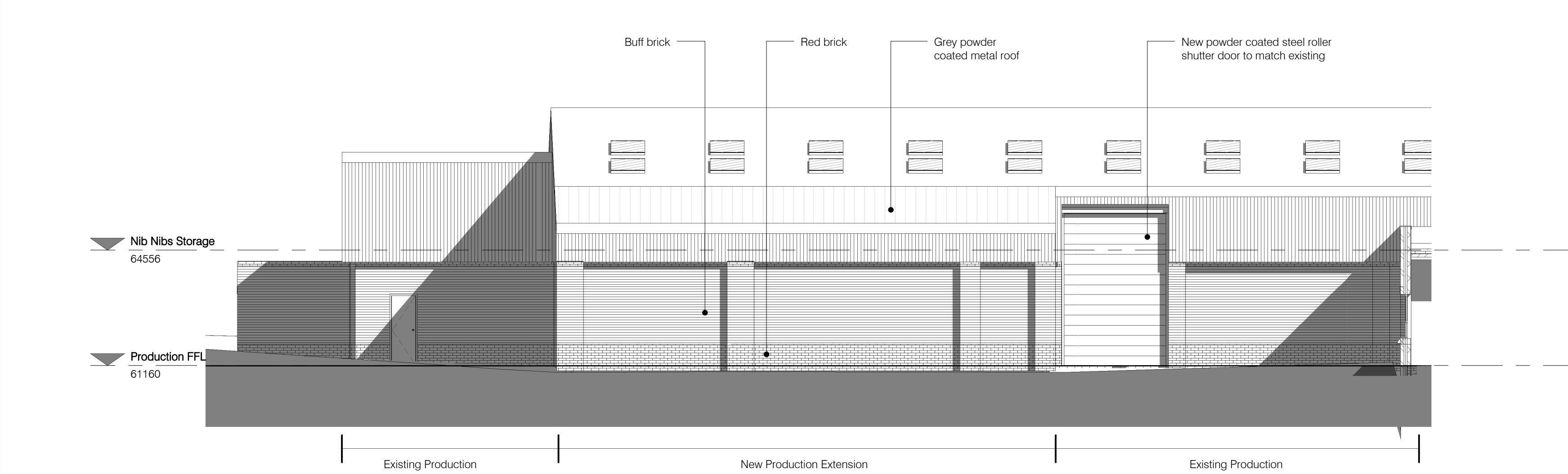
Elevation 5 - East Elevation Part 2 1 : 100
