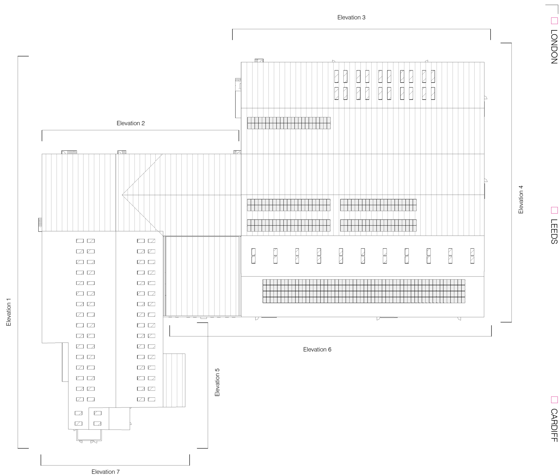
Elevation Key Plan 1 : 500
