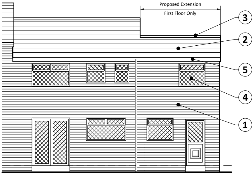
REAR ELEVATION
