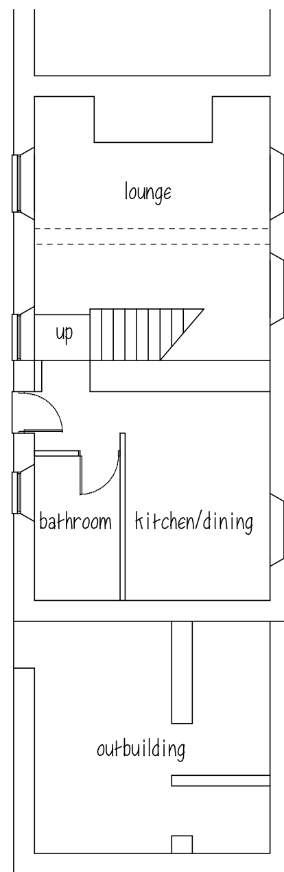
GROUND FLOOR
