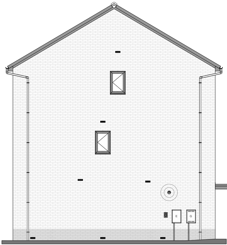
LEFT ELEVATION
