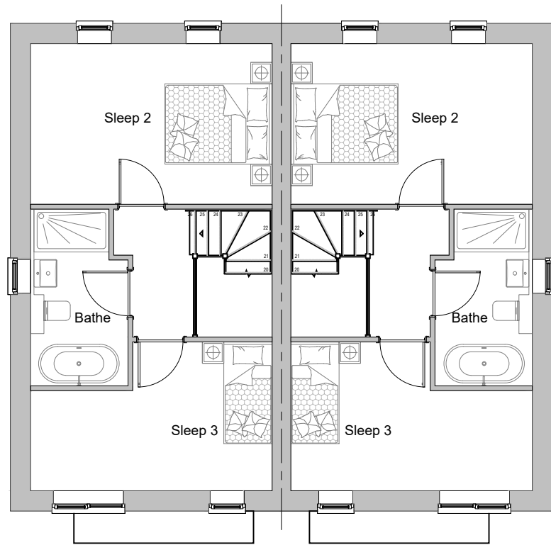
SECOND FLOOR
