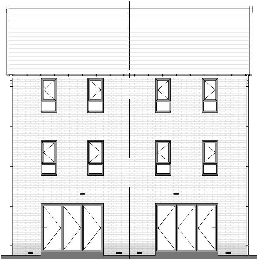
REAR ELEVATION
