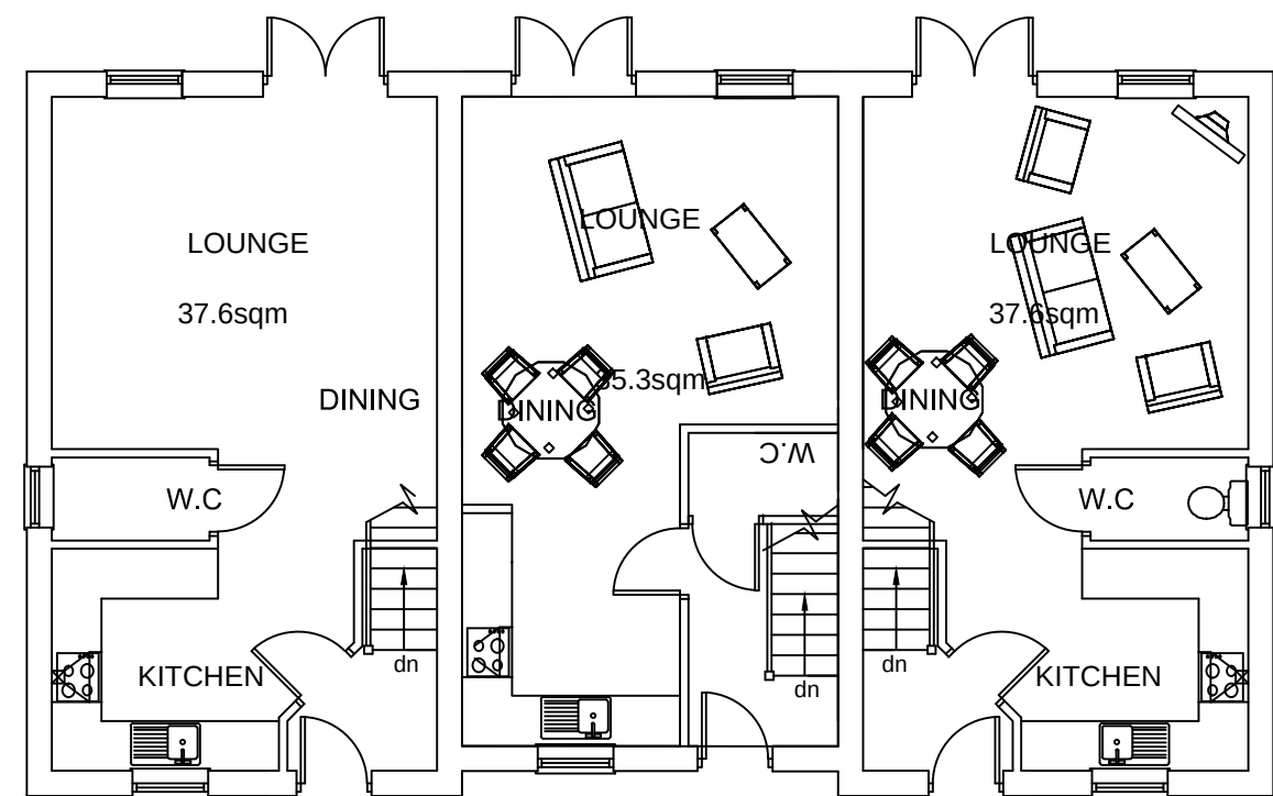
GROUND FLOOR PLAN PLOTS 1-6
