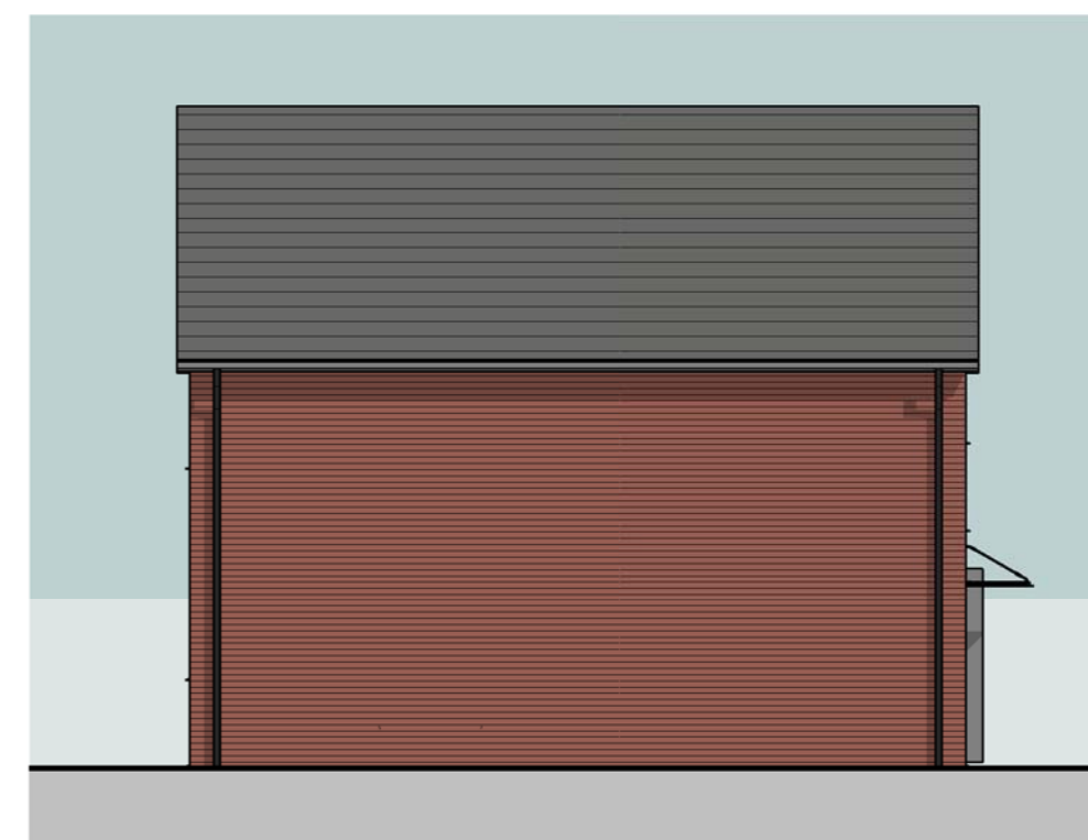
Plot 14 Side / East Elevation 1 : 100
