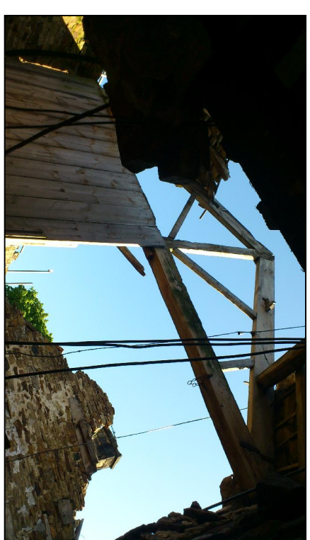
PICTURE H TRUSS REFERRED TO IN PICTURE G ABOVE AND DETEIORATION OF EXPOSED MASONRY TO WALL TOP
