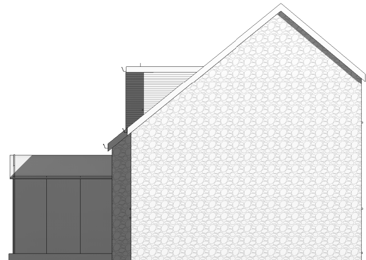
2 NORTH EAST 1 : 100
