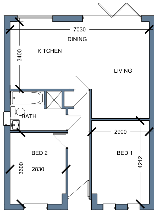
PLAN
