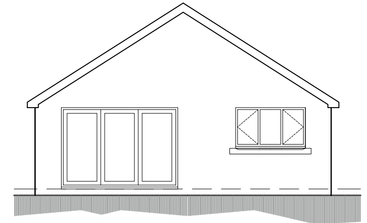
REAR ELEVATION
