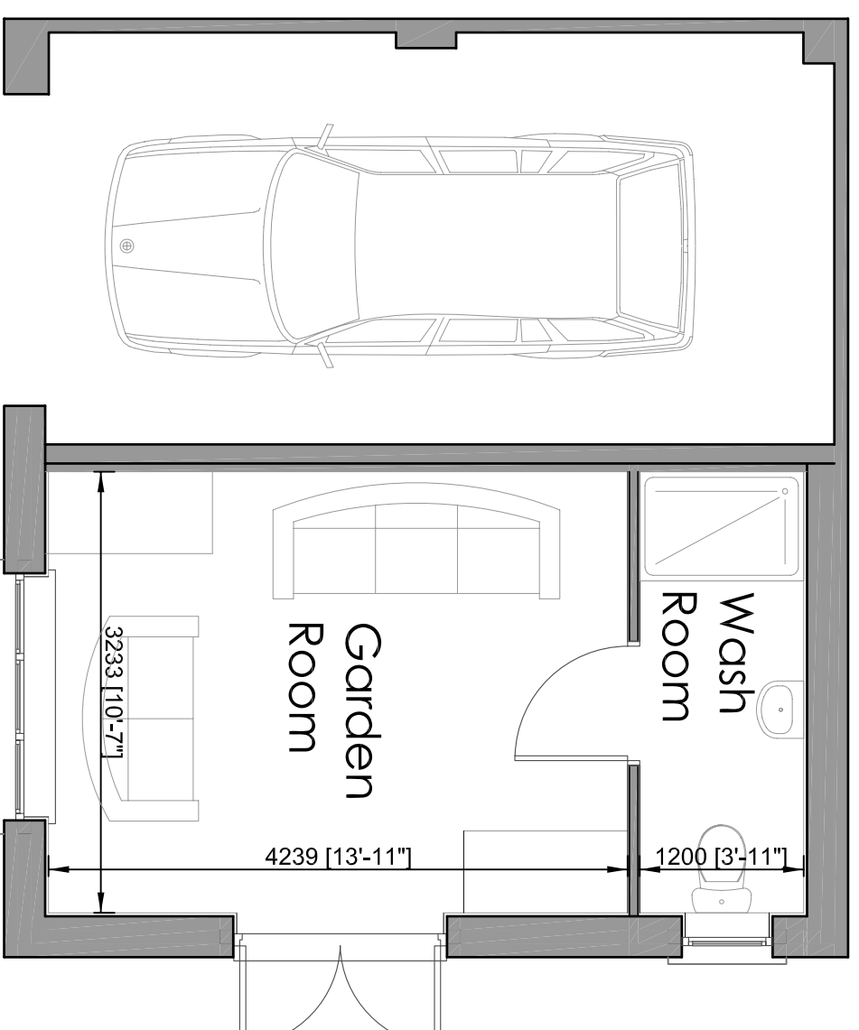
Floor Plan
