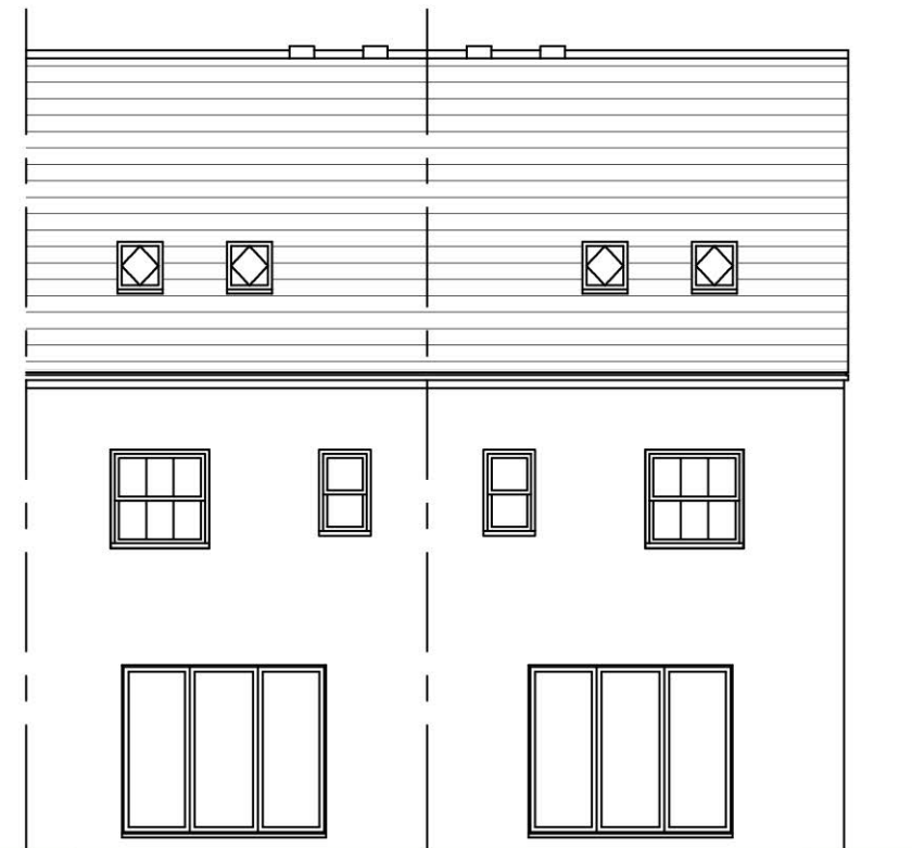
REAR ELEVATION TYPE J - MID
