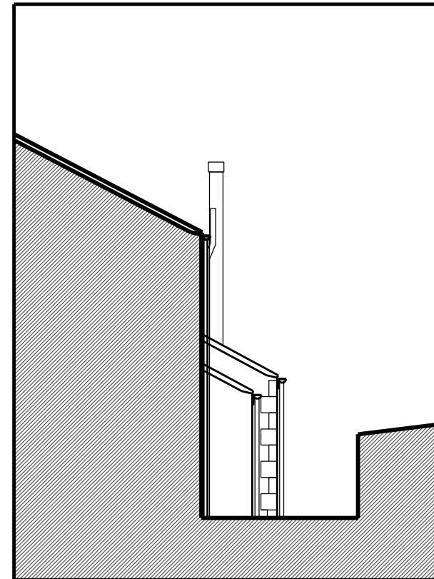
West Elevation - Proposed
