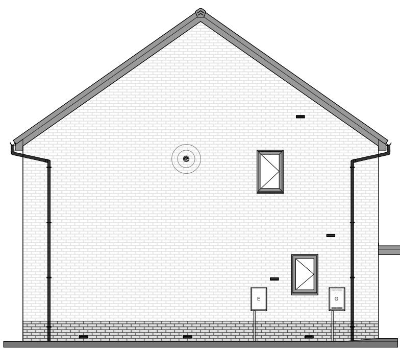
LEFT ELEVATION
