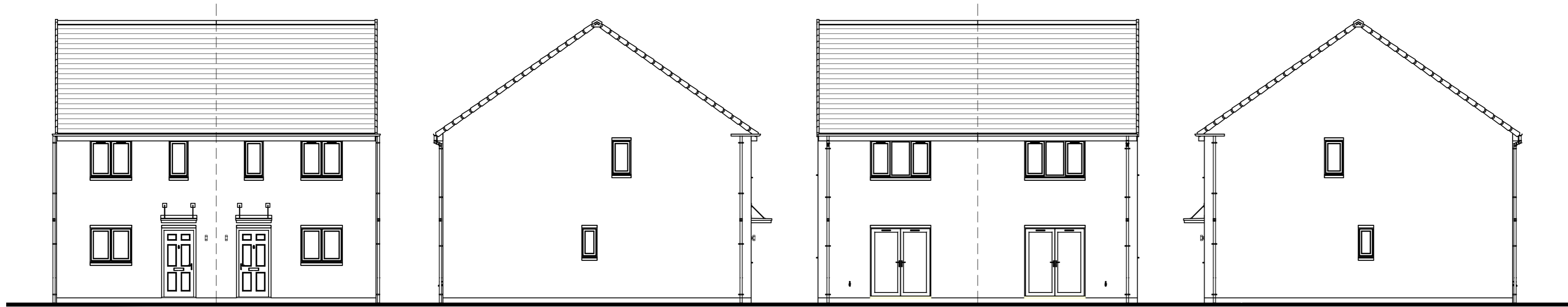
FRONT ELEVATION
