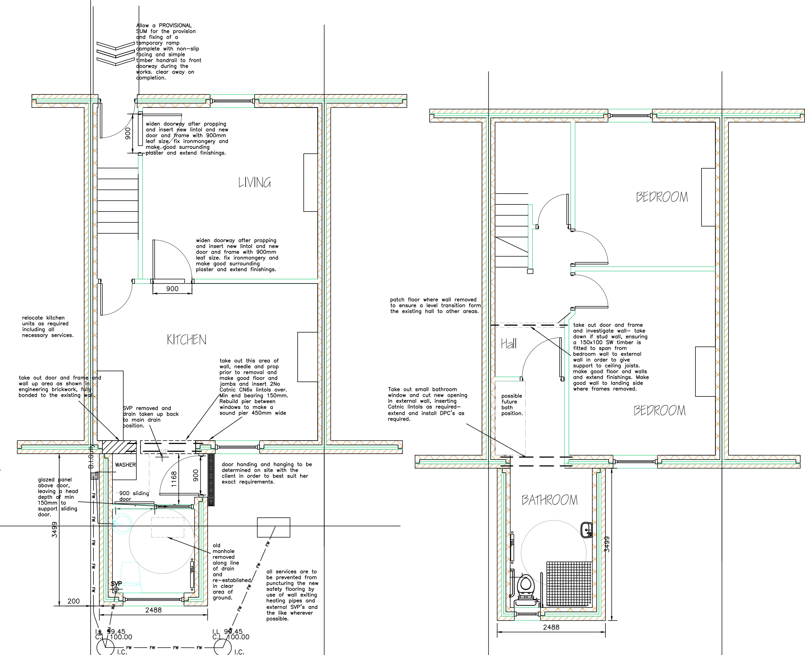
PROPOSED GROUND FLOOR PLAN PROPOSED FIRST FLOOR PLAN
